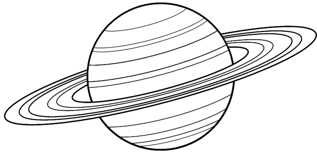
Saturn
