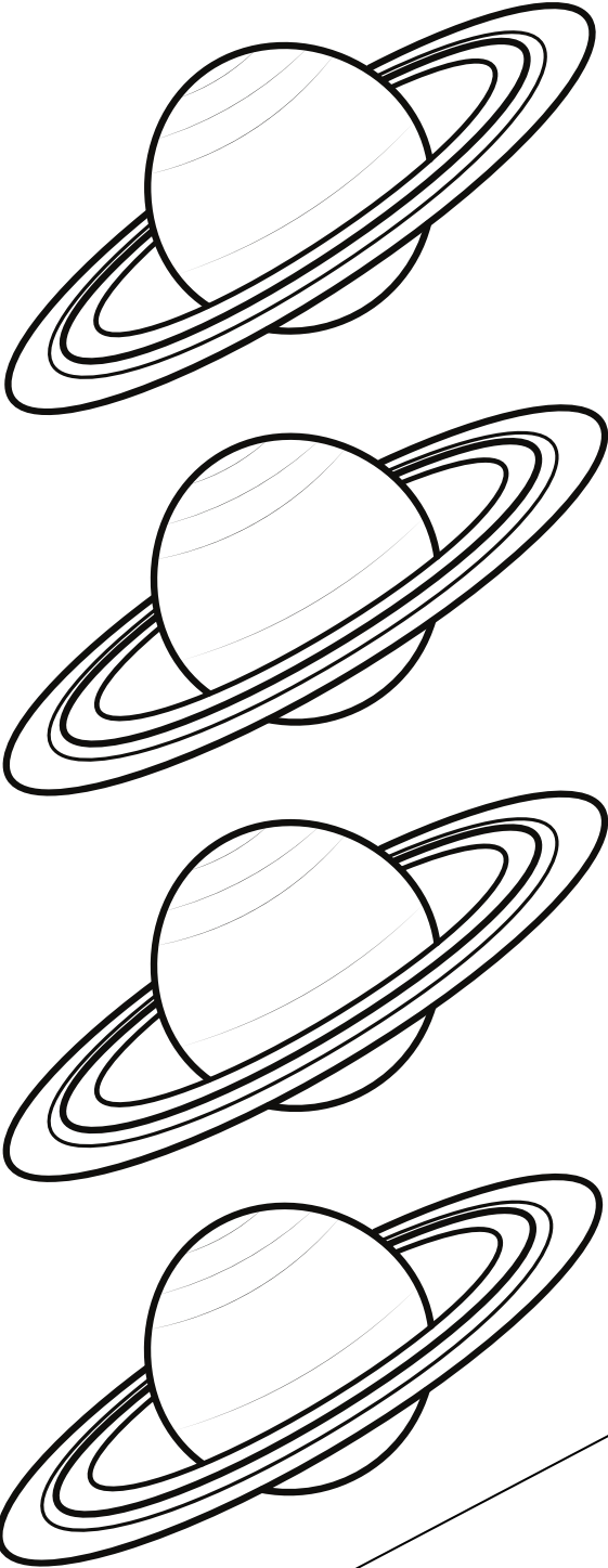
Saturn
